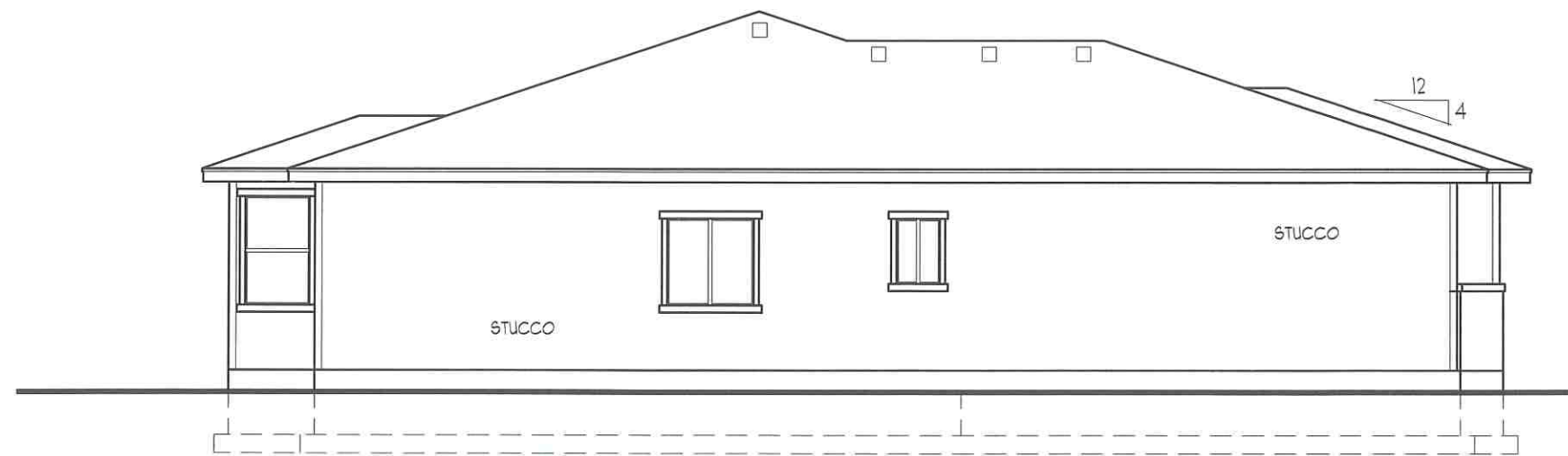
LEFT ELEV. VIEW SCALE 1/8" = 1'-0"
